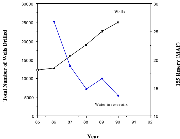
Figure 1: Water in Reservoirs and Wells Drilled during the 1987-1992 Drought
